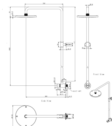
MODEL : FJHDS-115HFS Self Closing Shower Set
